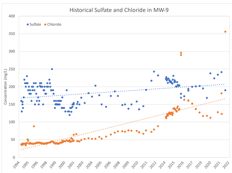
Sulfate and Chloride in Groundwater, MW-9. 1994-2022
