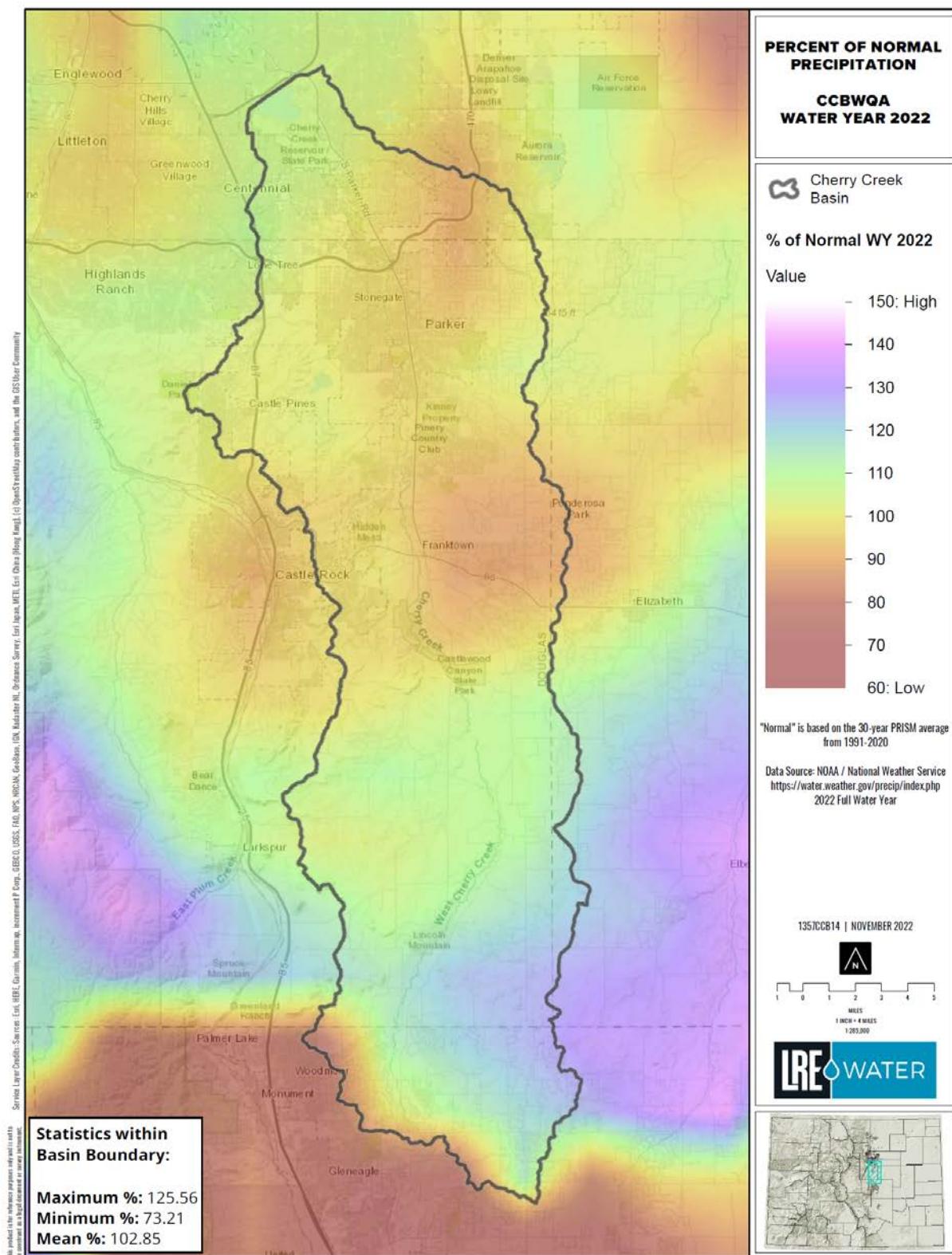
Figure 5. Percent of Normal Precipitation in the Cherry Creek Basin based on 30-year PRISM normal (1991-2020).
