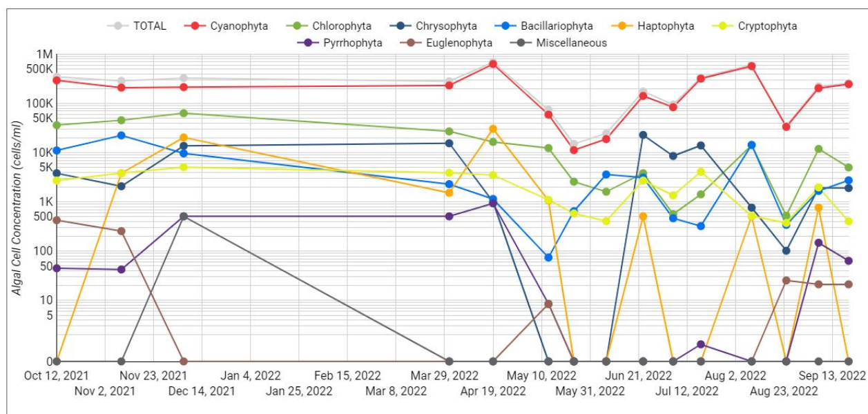
Figure 55. Phytoplankton Concentrations in Cherry Creek Reservoir, WY 2022.
