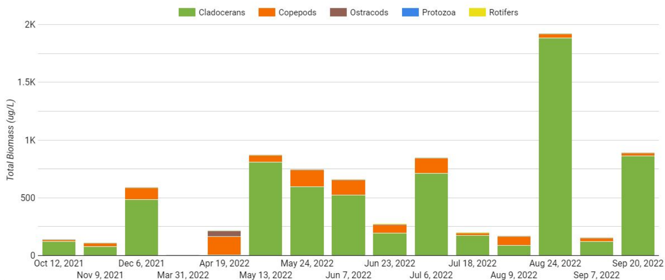
Figure 60. Total Zooplankton Biomass (µg/L) in WY 2022.
