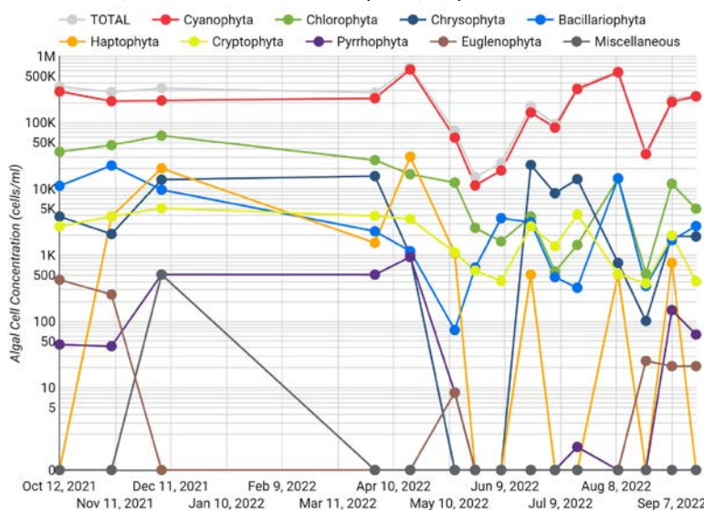
Phytoplankton Populations in CCR during WY 2022.
